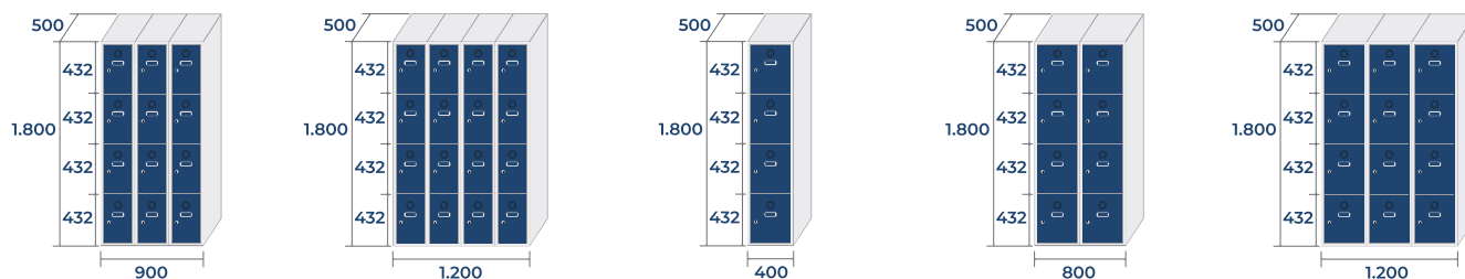
ECOC-30/3 PRO 54,9kg . 0,81m 3 ECOC-30/4 PRO 71,2kg . 1,08m 3 ECOC-40/1 PRO 25,7kg . 0,36m 3 ECOC-40/2 PRO 45,4kg . 0,72m 3 ECOC-40/3 PRO 65,1kg . 1,08m 3
