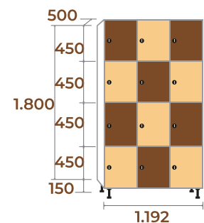
MHC-40/3 | MHFC-40/3 106kg | 115kg . 1,07m 3
