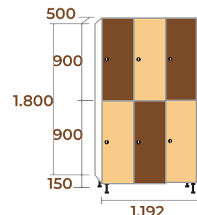
MHT-40/3 | MHFT-40/3 90kg | 99kg . 1,07m 3
