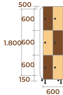
MHM-30/2 | MHFM-30/2 60kg | 64kg . 0,54m 3
